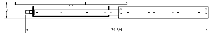
16", 150# Slides
