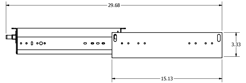
14" 250# Class Slide
